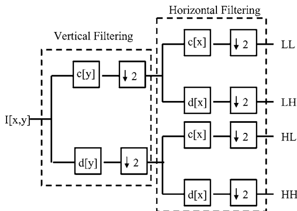
Figure 16. One stage in a filter-bank wavelet decomposition.
