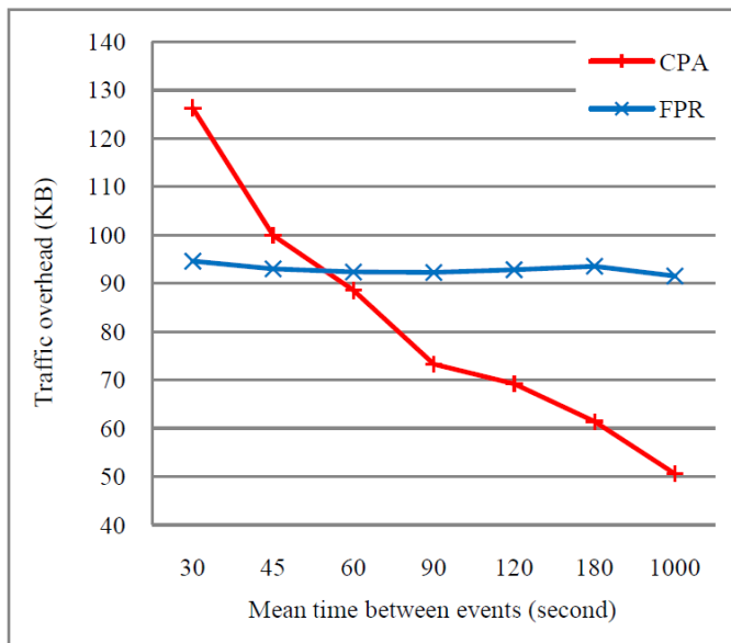
Fig. 5: Simulation results
