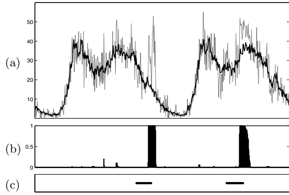
Figure 14: (a) Data for May 17-18, 2005, along with rate \lambda(t) ; (b) probability of event p(z) ; (c) actual event times.
