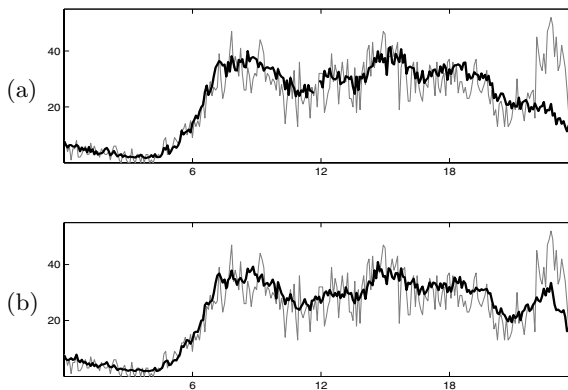
Figure 2: Example of freeway traffic data for Fridays for a particular on-ramp. (a) Average time profile for normal, non game-day Fridays (dark curve) and data for a particular Friday (6/10/05) with a baseball game that night (light curve). (b) Average time profile over all Fridays (dark curve) superposed on the same Friday data (light curve) as in the top panel.
