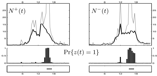
Figure 12: Data for Oct. 3, 2005, along with rate \lambda(t) and probability of event p(z) . At 3:30 P.M. an event was held in the building atrium, causing anomalies in both the incoming and outgoing data over most of the time period.
