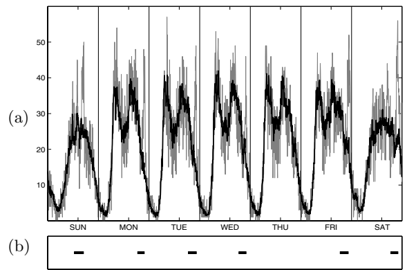
Figure 4: (a) One week of traffic data (light curve) from Sunday to Saturday (June 5-11), with the estimated normal traffic profile (estimated by the proposed model described later in the paper) superposed as a dark curve. (b) Ground truth list of events (baseball games).
