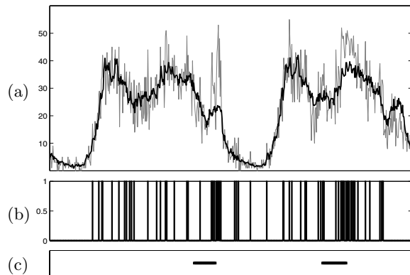
Figure 6: Same as Figure 5 but with an even lower threshold to detect the full duration of the large event on the second day, causing multiple false alarms.
