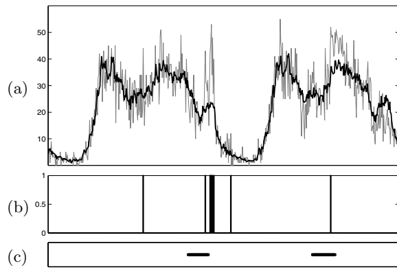
Figure 5: Illustration of the baseline threshold model set to detect the event on the second day, with (a) original freeway traffic time series in the top panel (light curve) for May 17-18, and mean profile as used by the threshold model (dark curve), (b) events detected by the threshold method in the center panel, and (c) ground truth (known events) in the bottom panel. Note the false alarms.
