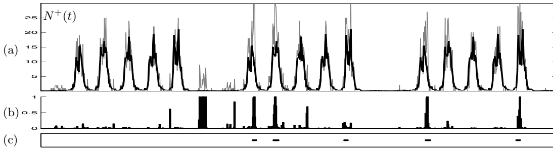
Figure 11: (a) Entry data, along with \lambda(t) , over a period of three weeks (Sept. 25–Oct. 15). Also shown are (b) the posterior probability of an event, p(z) , and (c) the periods of time in which an event was scheduled for the building. Most of the scheduled events are detected, along with a few other time periods (such as a period of greatly heightened activity on the first Saturday).
