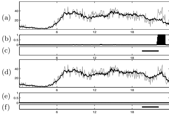
Figure 13: A Friday evening game, Apr. 29, 2005. Shown are (a) the prediction of normal activity, \lambda(t) ; (b) the estimated probability of an event, p(z) ; and (c) the actual game time. Panels (d)-(f) show the threshold model's prediction for the same day.
