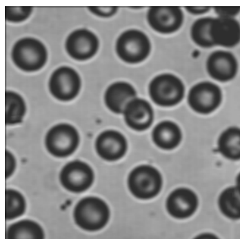
Filtered Image
