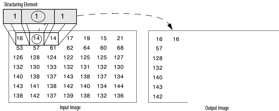
Figure 9-2: Morphological Processing of Grayscale Images
