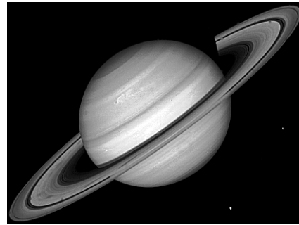
Sharpened Image
