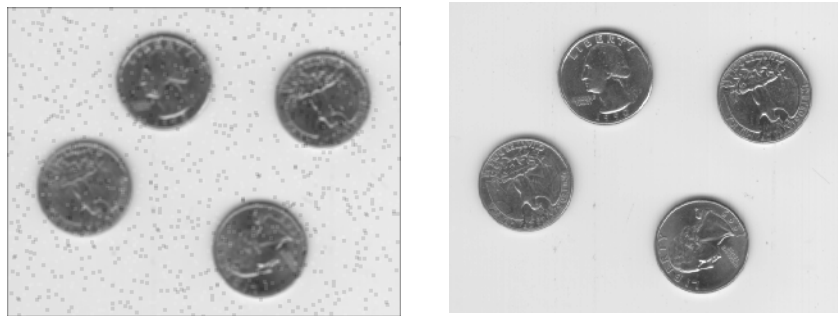
Averaging Filter
