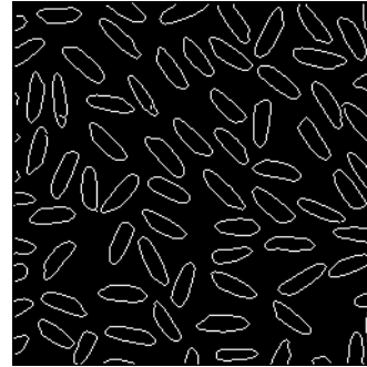
Canny Filter
