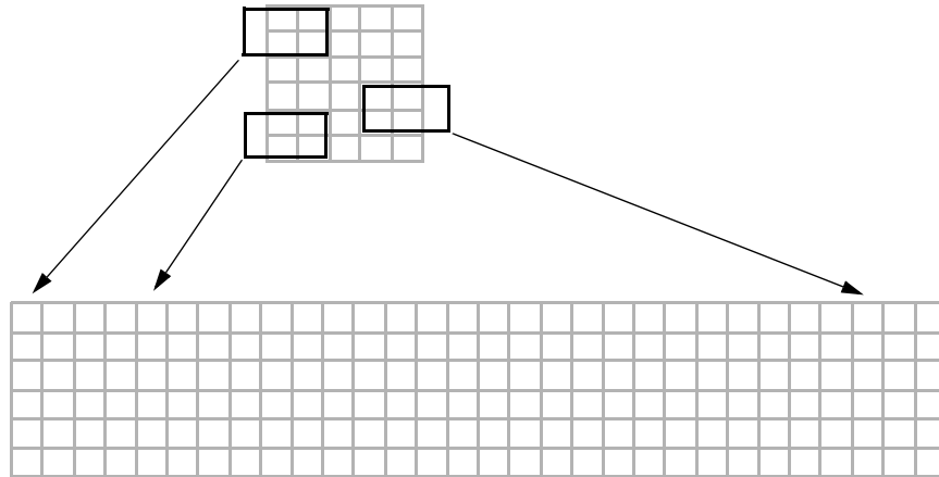
Figure 6-5: colfilt Creates a Temporary Matrix for Sliding Neighborhood
