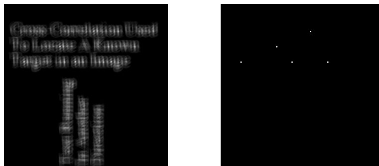
Figure 8-9: A Correlated Image (left) and its Thresholded Result (right)
