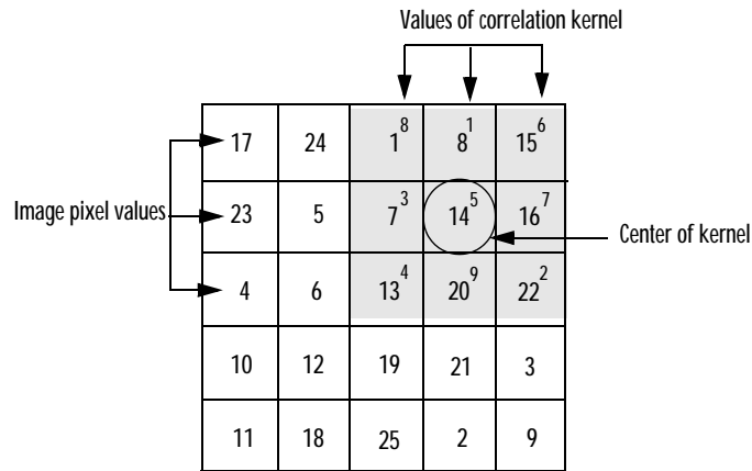
Figure 7-2: Computing the (2,4) Output of Correlation
