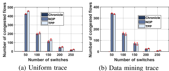
Fig. 15. Number of congested flows with different numbers of switches.
