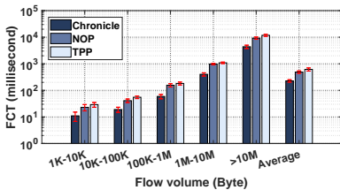
Fig. 11. FCT for data mining trace.
