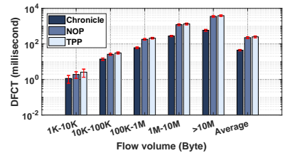
Fig. 13. DFCT with larger link delay.
