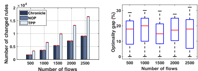
Fig. 20. Number of changed rules.
