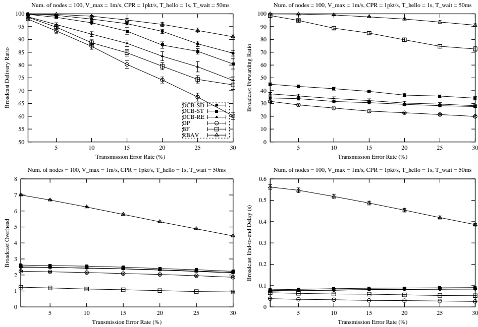
Fig. 5. Sensitivity to transmission error rate of the network: (a) delivery ratio, (b) forwarding ratio, (c) overhead and (d) end-to-end delay.
