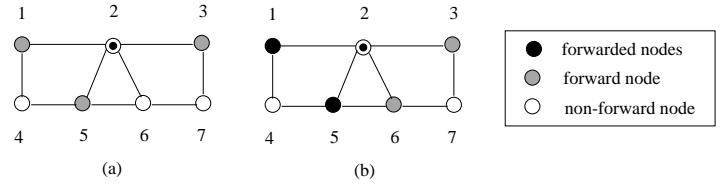
Fig. 2. A sample network where the node 2 uses the FNSSP to select its forward nodes in (a) case 1 and (b) case 2.
