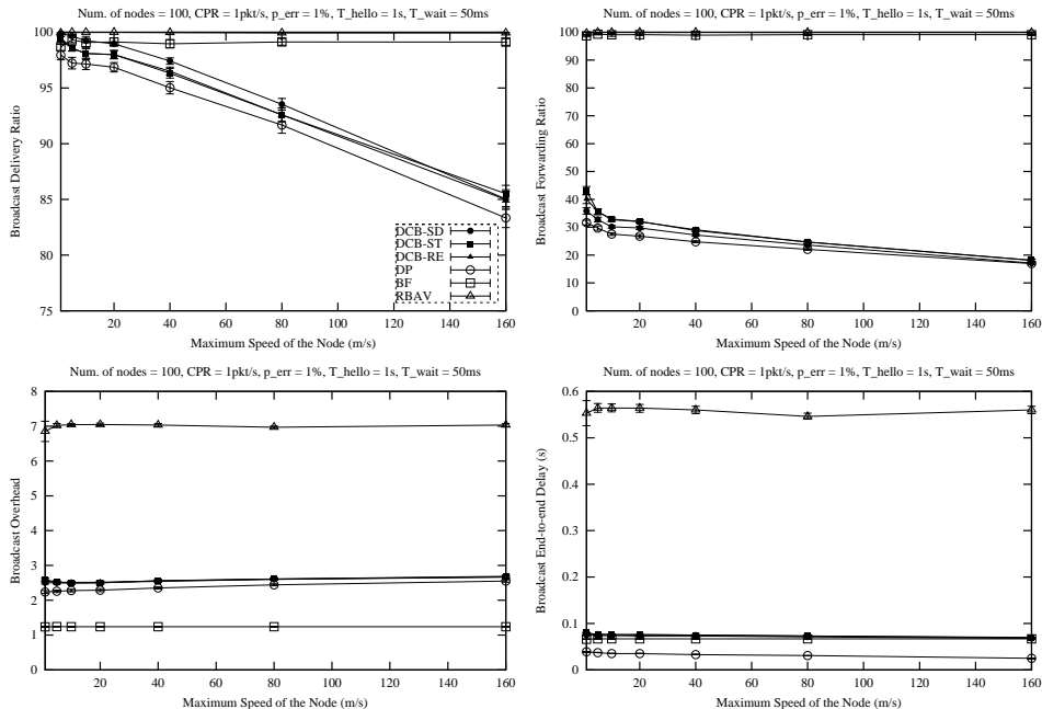
Fig. 6. Sensitivity to mobility of the node: (a) delivery ratio, (b) forwarding ratio, (c) overhead and (d) end-to-end delay.
