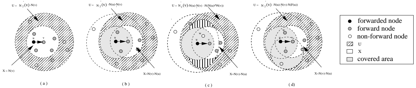
Fig. 1. Illustrations of four algorithms: (a) multiple relays (MPR), (b) dominant pruning (DP), (c) partial dominant pruning (PDP) and (d) CDS-based broadcasting (CDSB).
