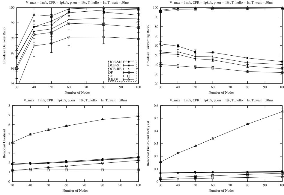
Fig. 4. Sensitivity to size of the network: (a) delivery ratio, (b) forwarding ratio, (c) overhead and (d) end-to-end delay.
