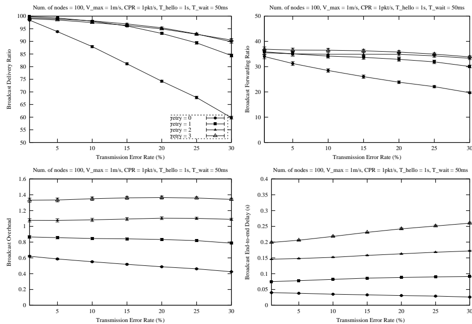
Fig. 7. Sensitivity to times of retry: (a) delivery ratio, (b) forwarding ratio, (c) overhead and (d) end-to-end delay
