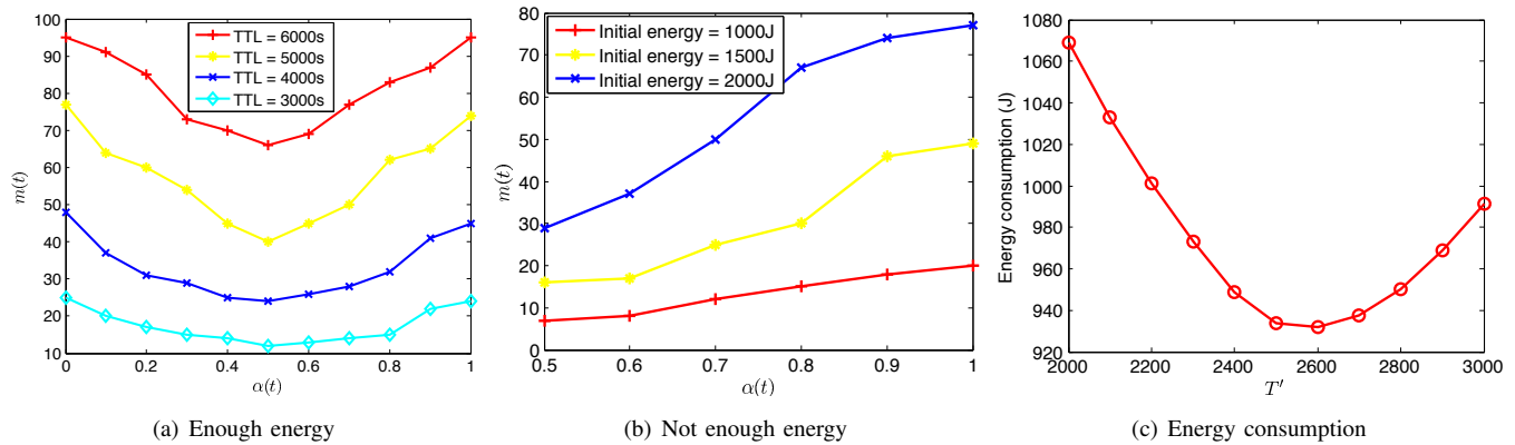
Fig. 7. The relationships among Energy consumption, m(t) and \alpha(t) under the random-waypoint mobility pattern.
