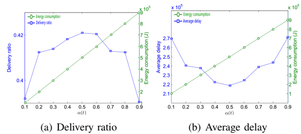
Fig. 11. Delivery ratio and Average delay as a function of \alpha(t) under the PMTR trace.
