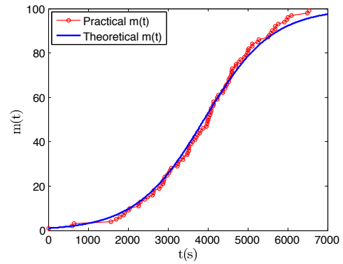
Fig. 8. The theoretical value and practical value of m(t) .
