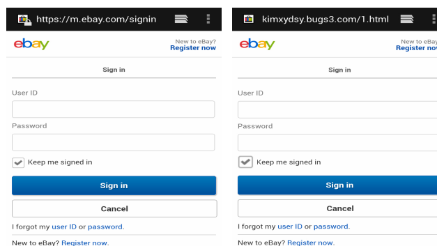
(a) Ebay Official Login Page (b) Ebay Phishing Login Page
