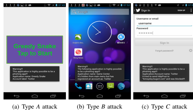
Fig. 13. Experiments with AccountFish
