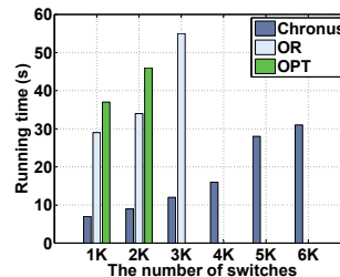
Fig. 10. Running time.
