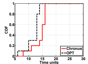
Fig. 11. Update time.
