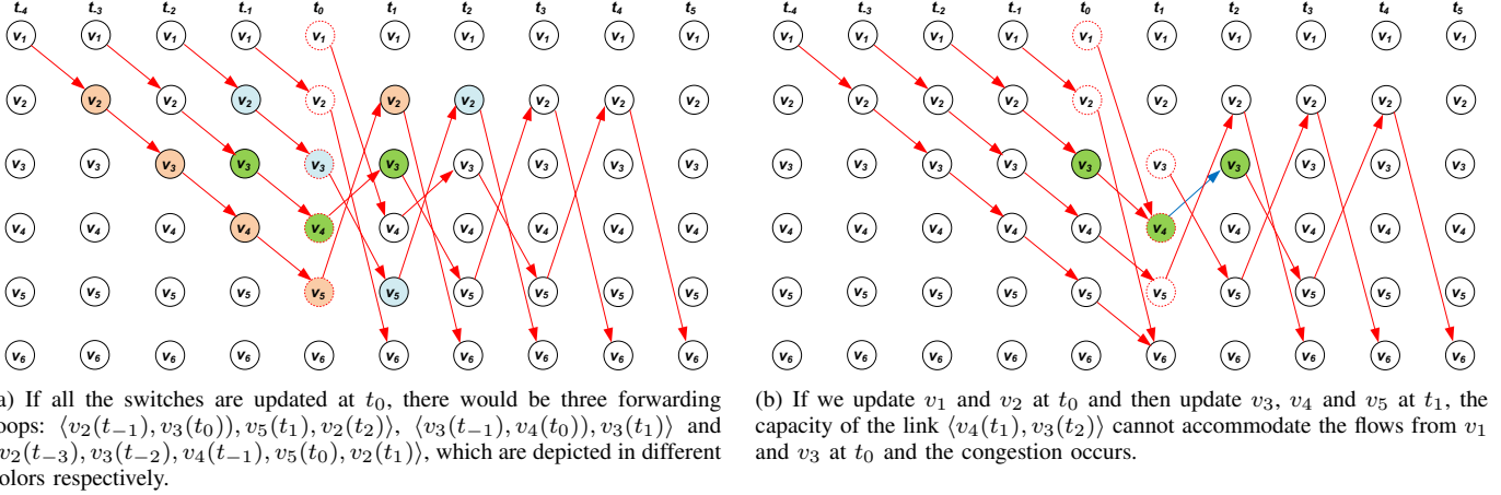
Fig. 2. Illustration of the different timed update sequences in the time-extended network.
