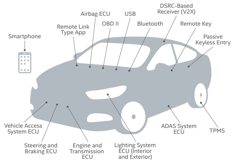
Fifteen of the most hackable and exposed attack surfaces, including several electronic control units, on a next-generation car.
